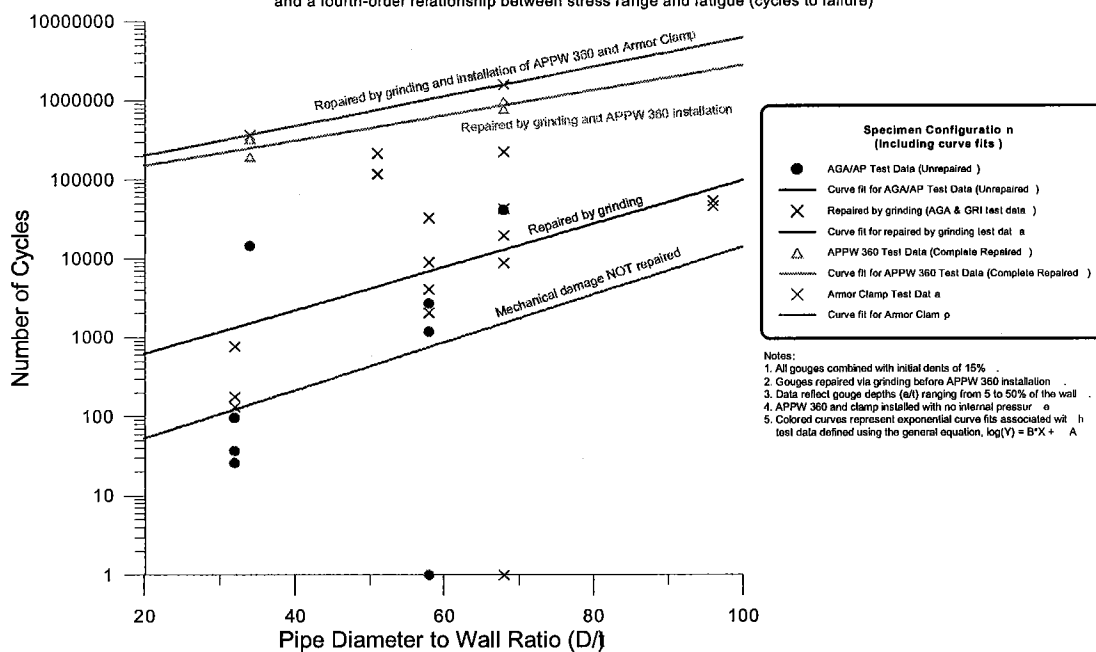
Figure 8 Fatigue data for dents and gouges in varying states of repair
