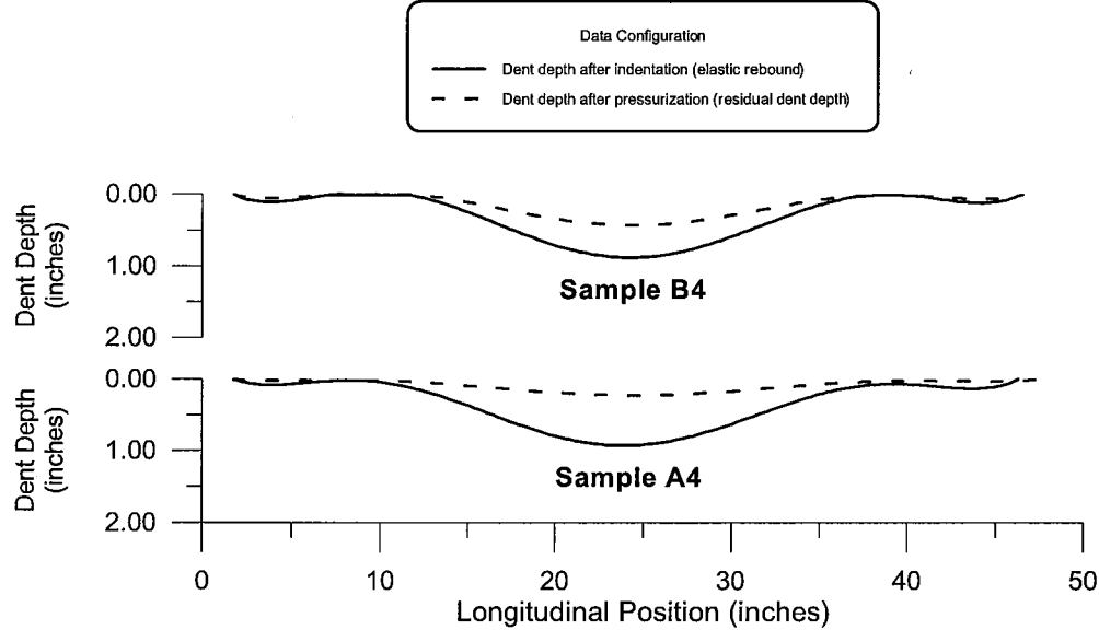
Figure 3 Profile of dent depth along longitudinal axis of pipe
