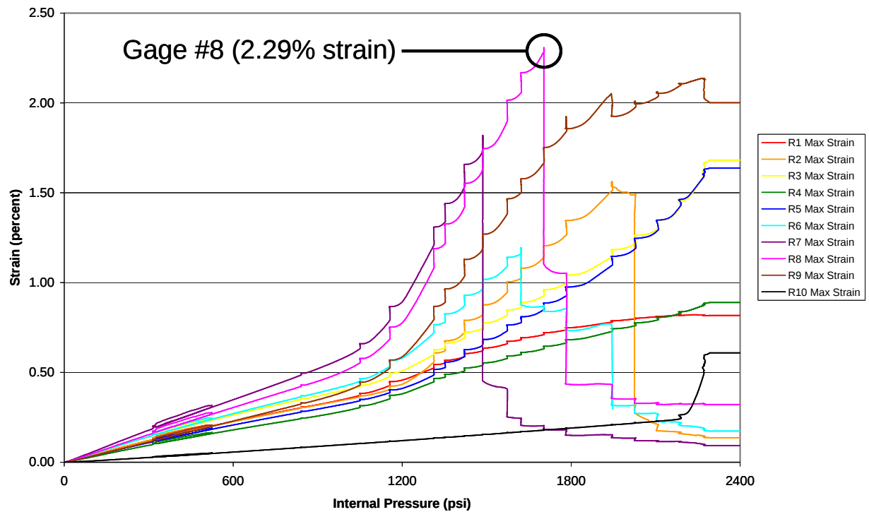
Figure 7 – Strain gages results for burst test (sample failed at 2,291 psi)
