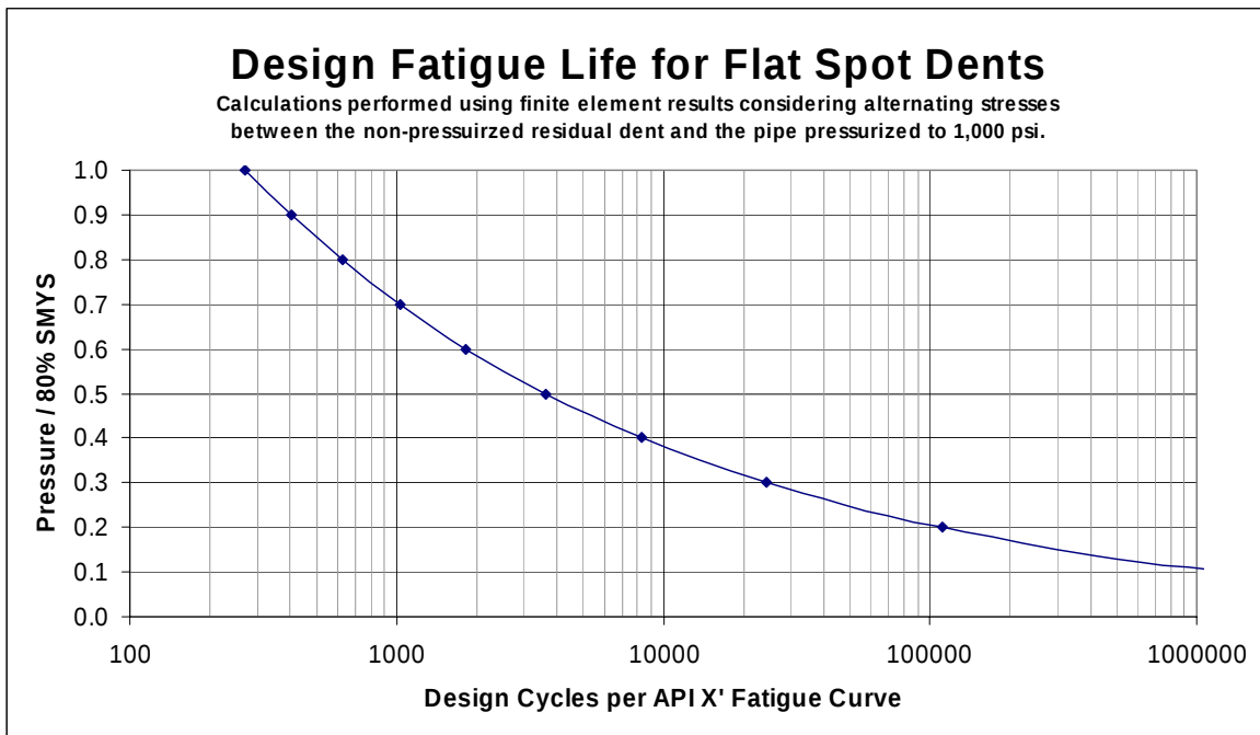
Figure 14 – Estimated design fatigue life based on FEA results (Test sample was subjected to 13,819 pressure cycles at 80% SMYS, DP = 100 to 1,168 psi, with NO failure in flat spot)
