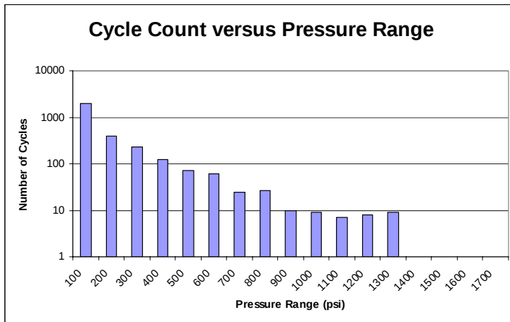
Figure 2 – Development of the histogram and single equivalent pressure range
